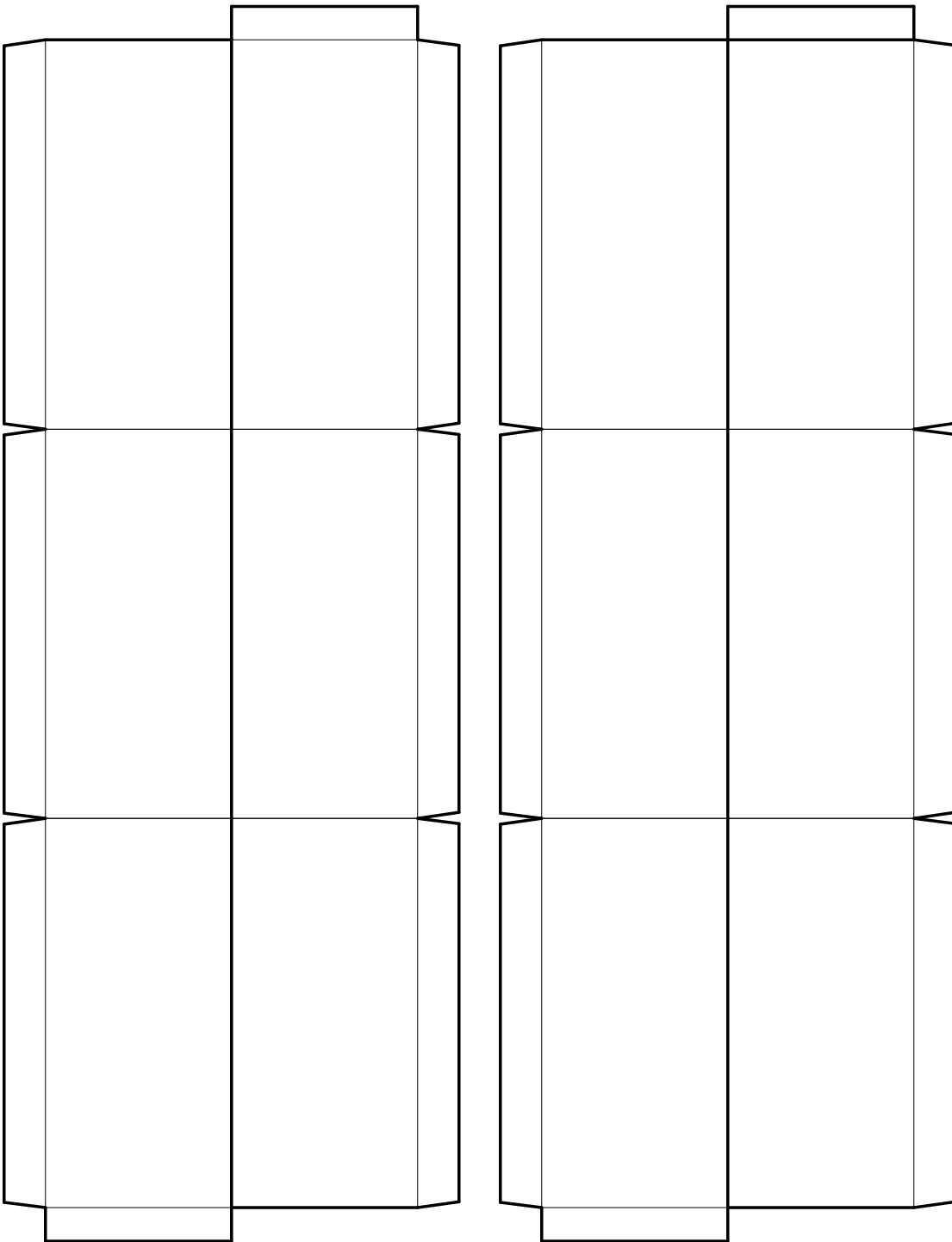
3ft riser wall @ 3/8''=1 ft. This pattern is for 12 riser panels. 20 panels will be needed for dome
